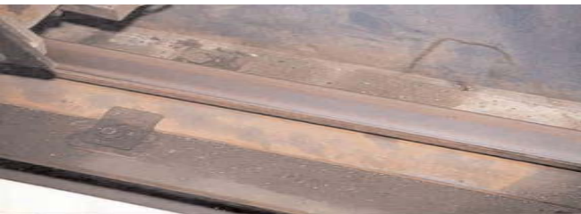
After Kelsan SL/SFM System: Metal flakes are gone, a sign that wheel/rail wear is significantly reduced.
