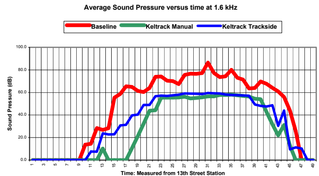
Fig 9. Time based squeal frequency response: 1.6 kHz
