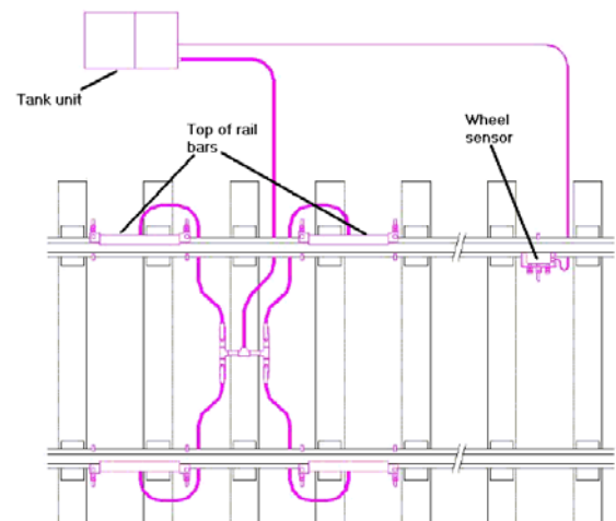
Fig 3. Schematic of trackside application layout
