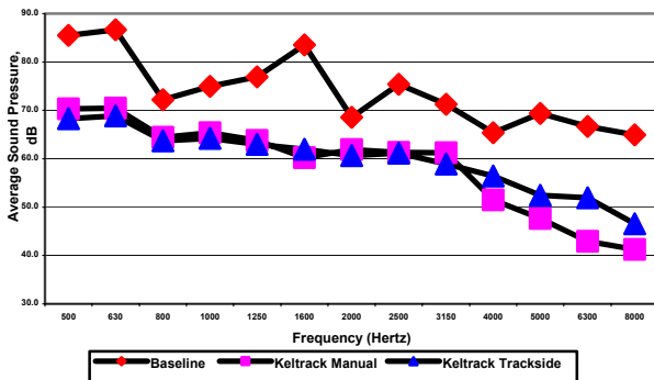
Fig 8. Average sound pressure versus frequency
