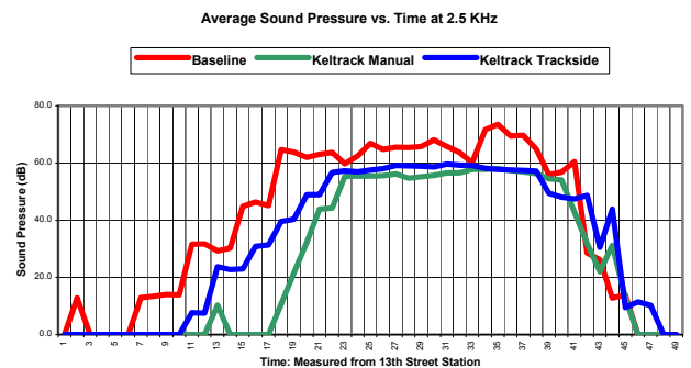
Fig 10. Time based squeal frequency response: 2.5 kHz
